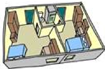
Floor plan of 2 bedroom unit Leggett/Watts
